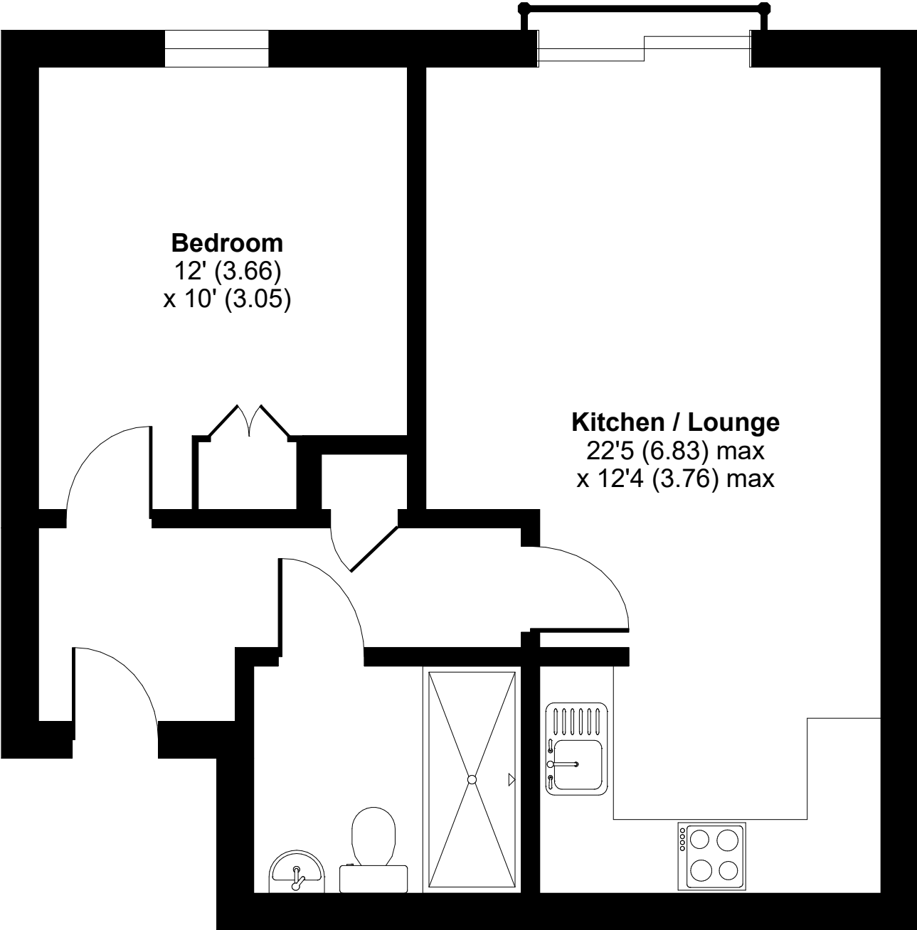
FIRST FLOOR
